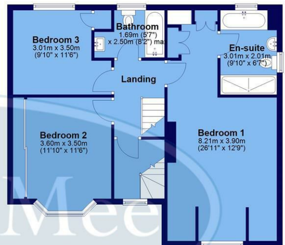
First Floor Approx. 69.1 sq. metres (744.3 sq. feet)
